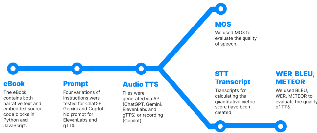
Figure 1: Evaluation workflow: eBook content was converted to audio via TTS systems and assessed using MOS for subjective quality and BLEU, WER, and METEOR for quantitative evaluation.
